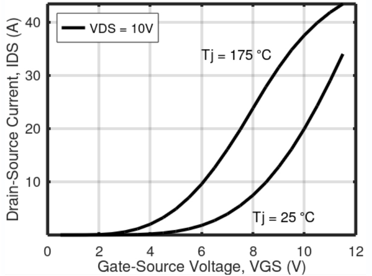
Figure 6: Transfer Characteristic
