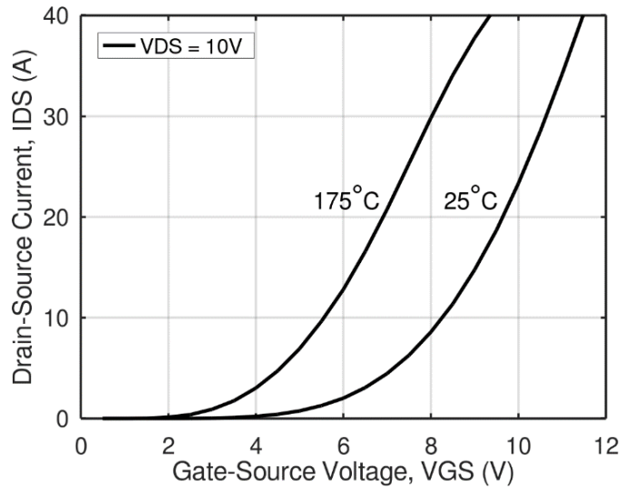
Figure 8: Biode Diode Characteristics. T J = 25, 175°C.
